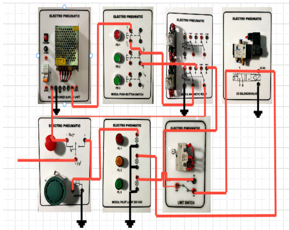
Gambar 2. Rangkaian elektronik cylinder single acting.
