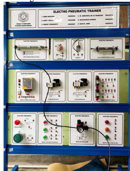
Gambar 1. Rangkaian pneumatik cylinder single acting.
