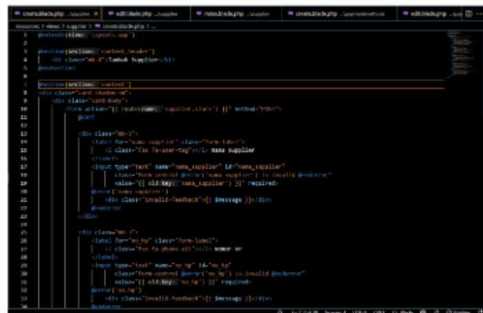
Gambar 41. Source Code Tambah Supplier
