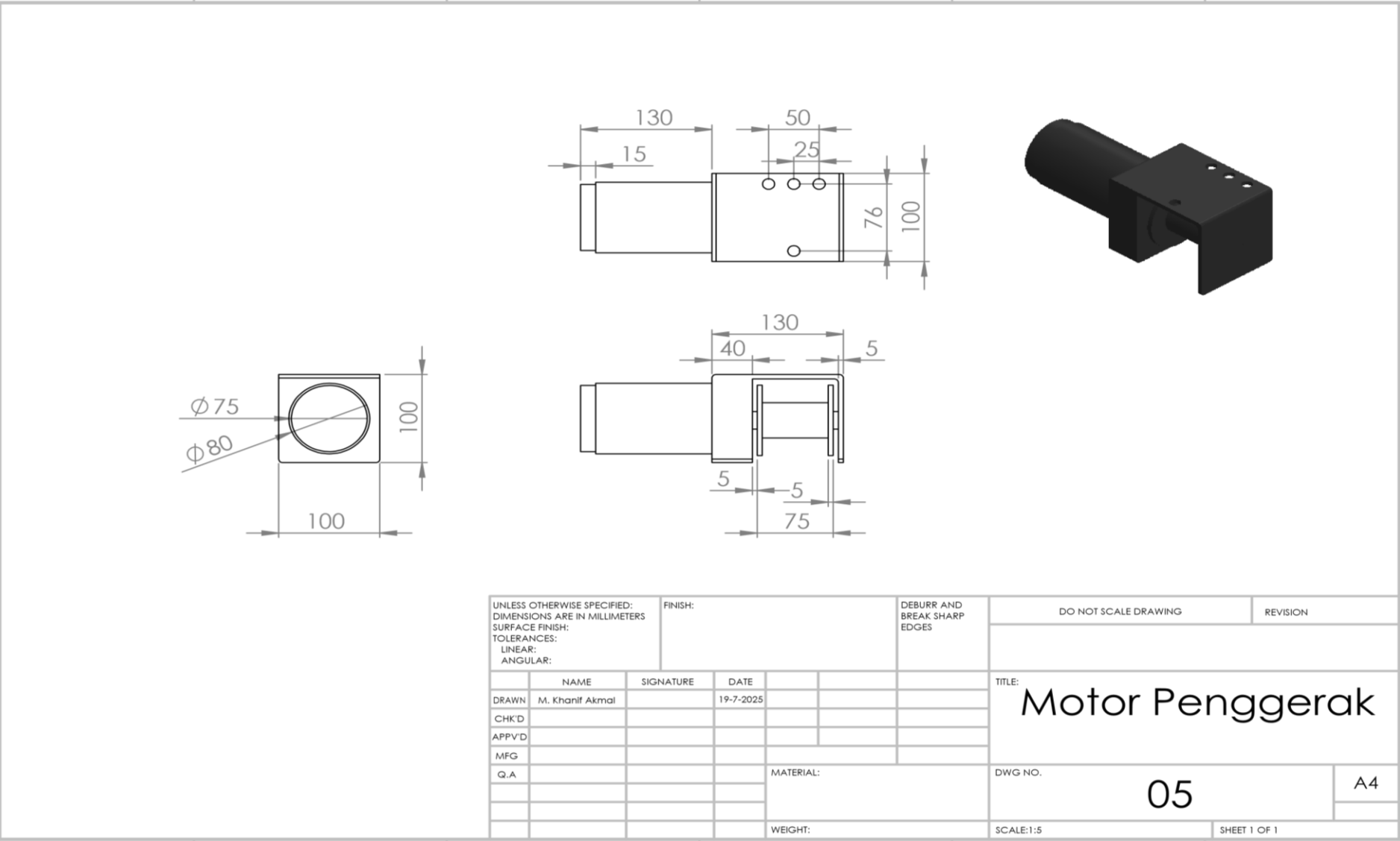
Lampiran 6 Gambar Kerja Winch
