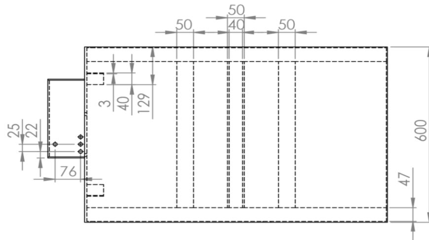
Lampiran 2 Gambar Kerja Platform Scissor Lift
