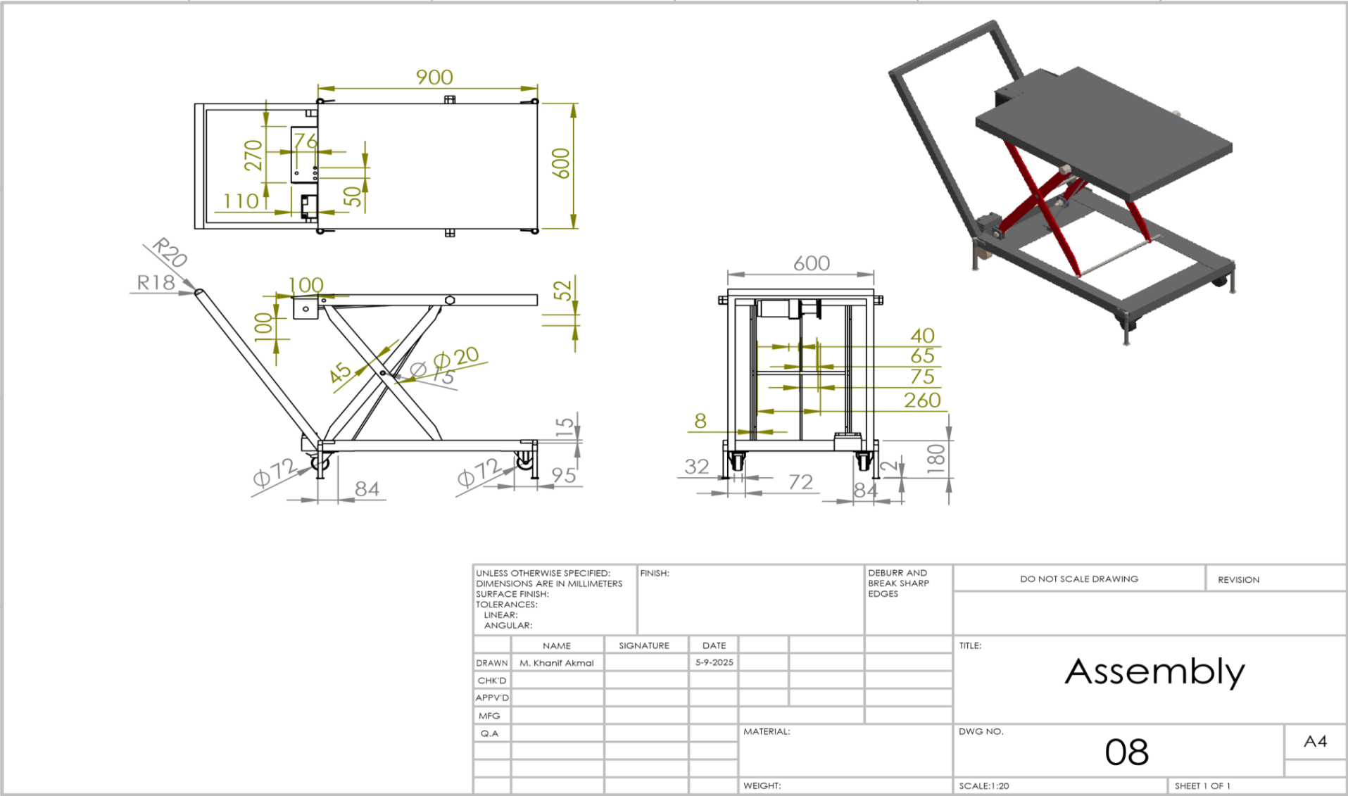
Lampiran 7 Gambar Kerja Scissor Lift Table
