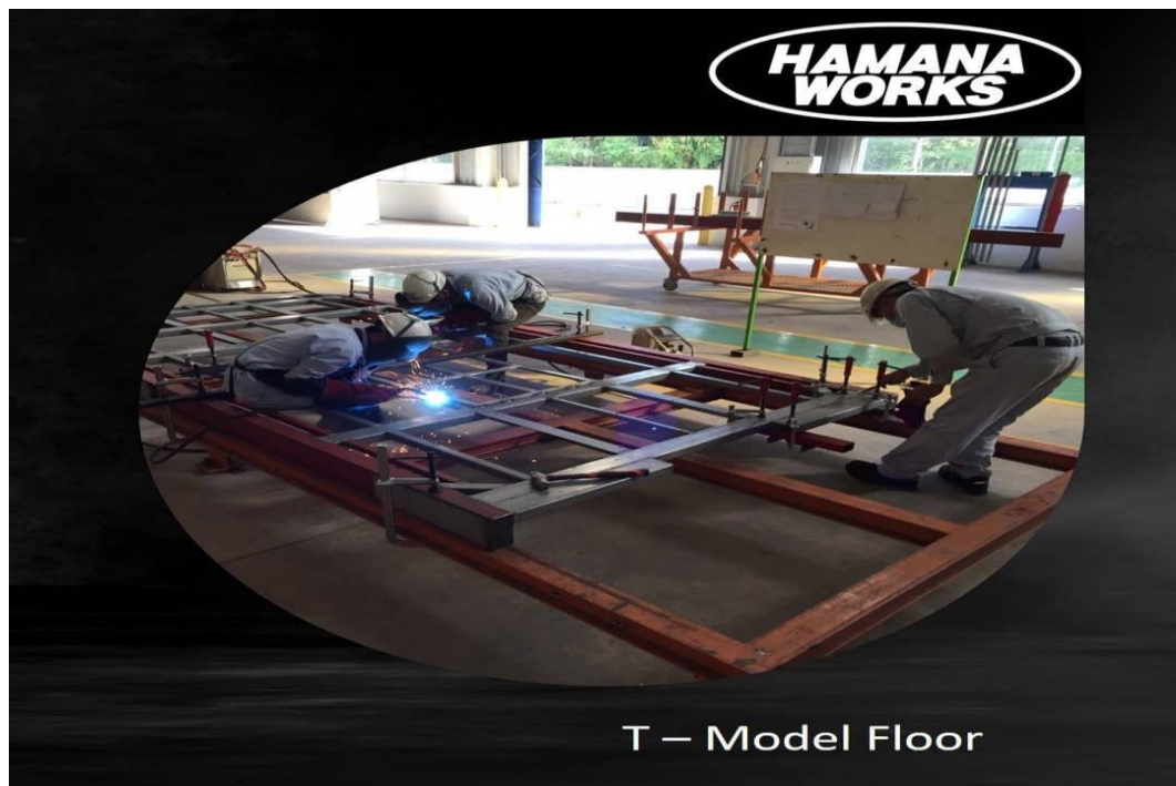
Lampiran 3. Proses Produksi Car Carrier di PT Hamana Works Indonesia
