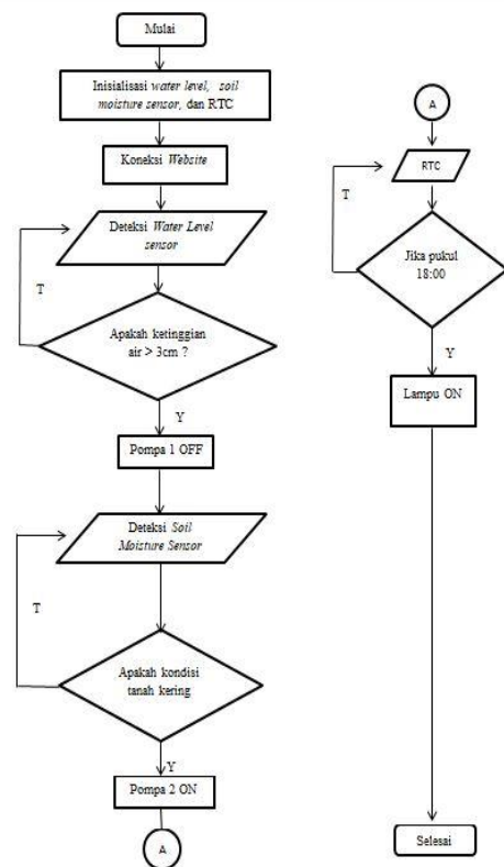
Gambar 1. Flowchart Alur Website
