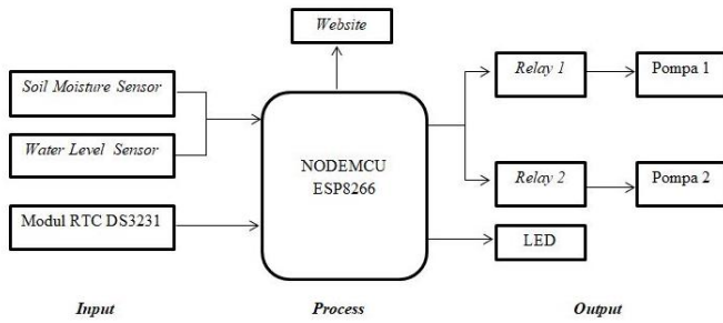
Gambar 2. Diagram Blok
