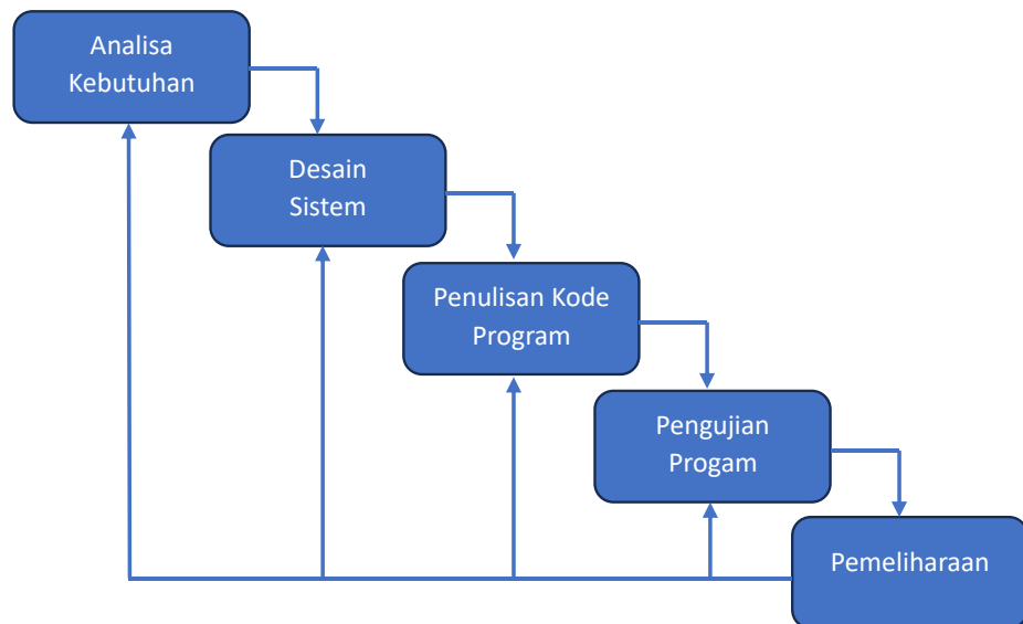
Gambar 3. 1 Metode Waterfall
