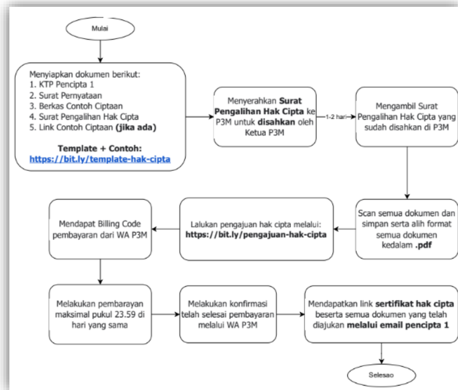
Gambar 3. 1. Proses HKI
